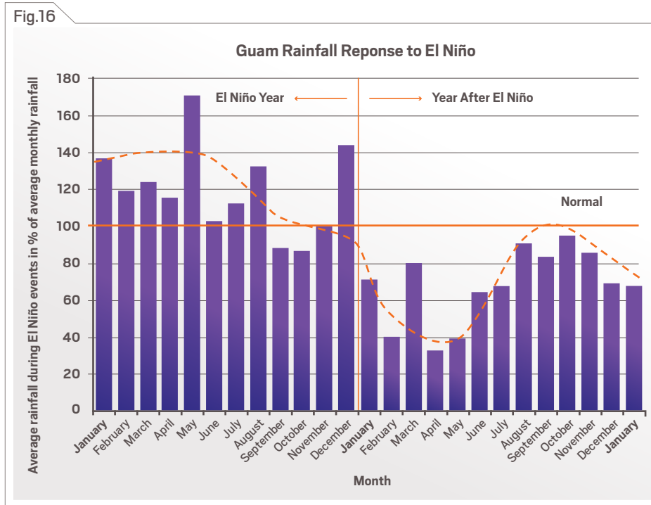
Figure 16. Average rainfall in Guam during El Niño events shown as the percent of average monthly rainfall. Source: Pacific ENSO Applications Climate Center 2018.
